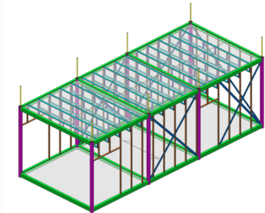
Figure 14: Structural design model of the module
