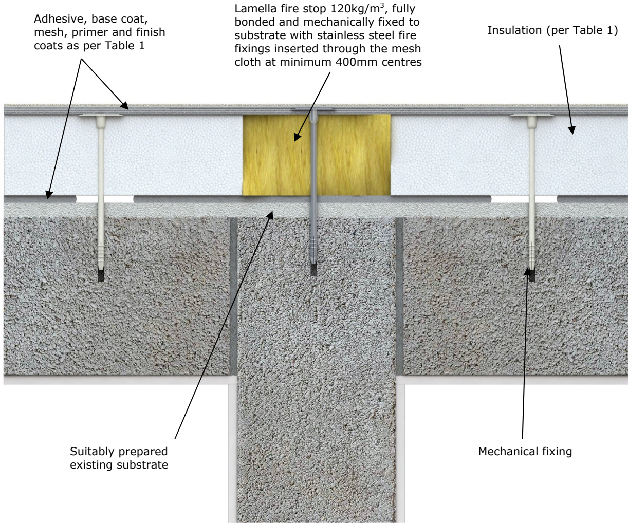
Figure 6: Firestop detail
