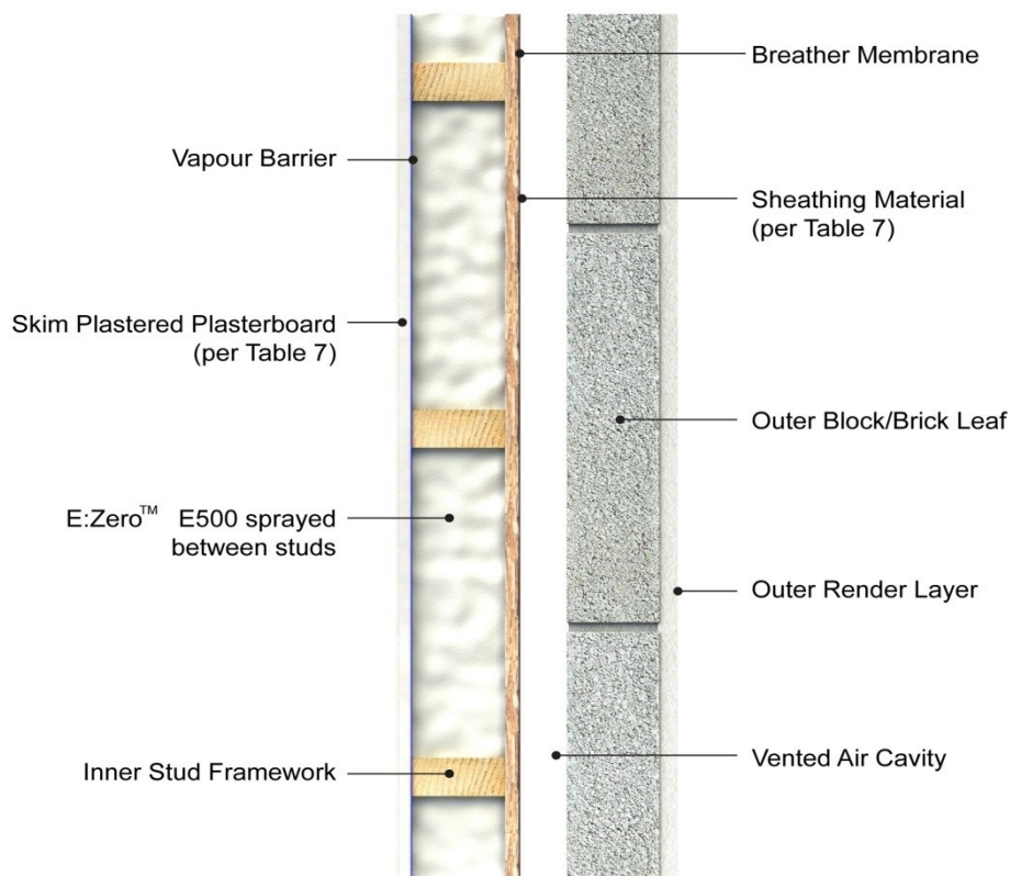
Figure 1: Timber Frame Wall
