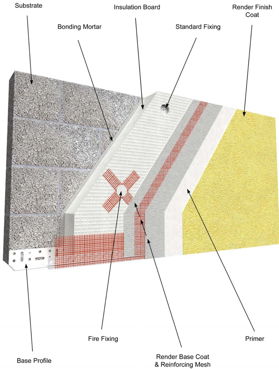
Figure 1: Baunit External Wall Insulation System – Isometric View
