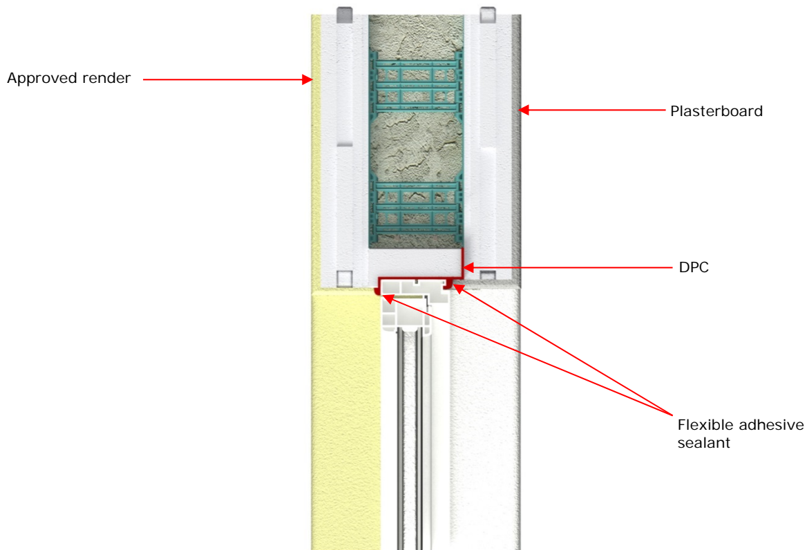
Figure 8: Header Detail
