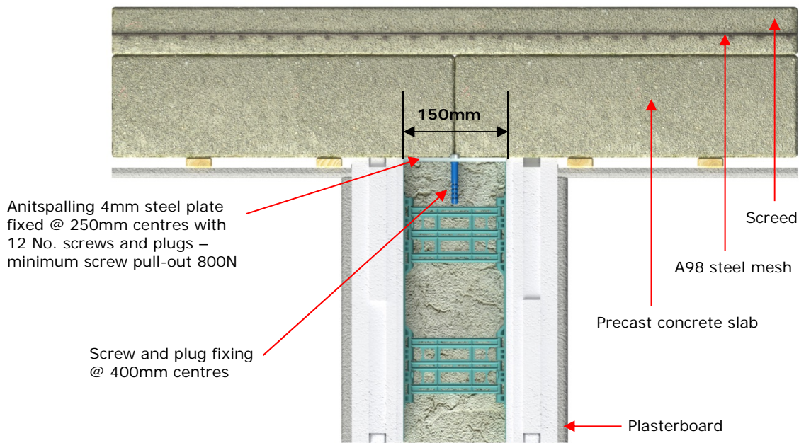
Figure 5: Internal Load Bearing Wall with Concrete Slab and Antisplalling Steel Plate
