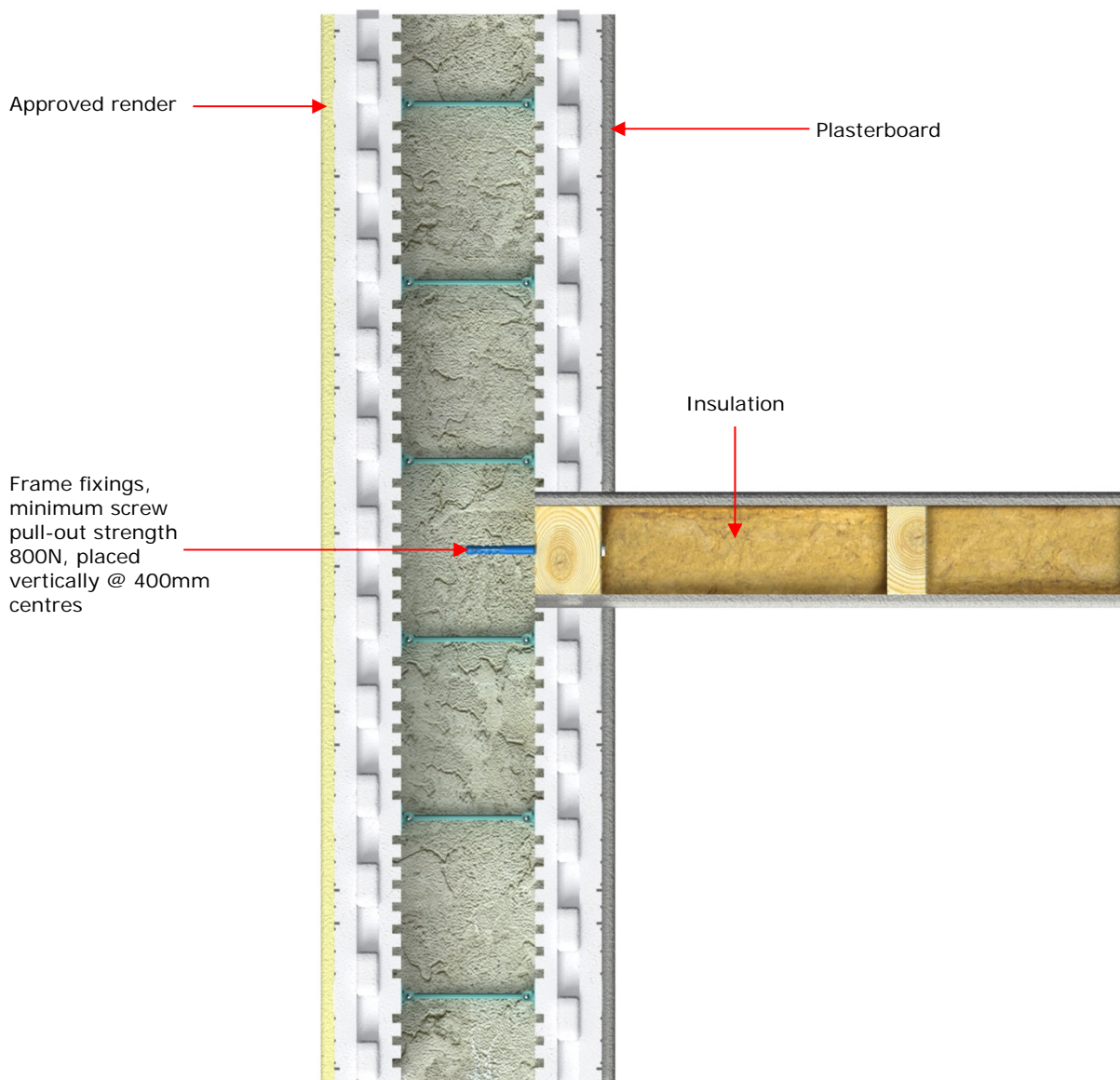
Figure 9: Internal Stooiling Wall with External Abutment
