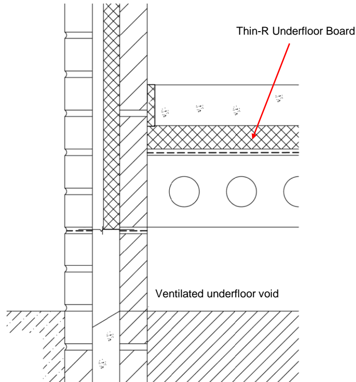
Figure 2: Suspended Concrete Ground Floor Detail
