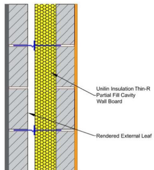
Figure 1: Unilin Cavity Wall Section
