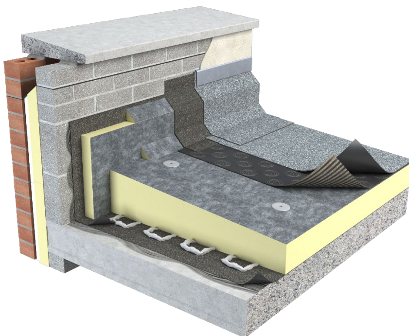
Figure 2: Unilin Insulation TR/BGM onto Concrete Deck
