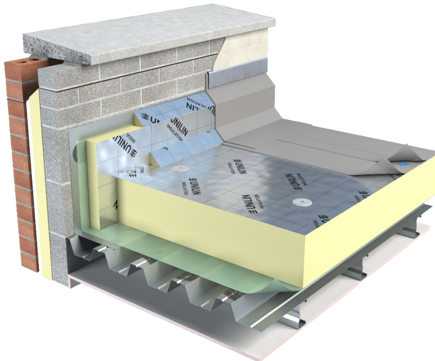
Figure 2: Unilin Insulation FR/ALU onto Metal Deck
