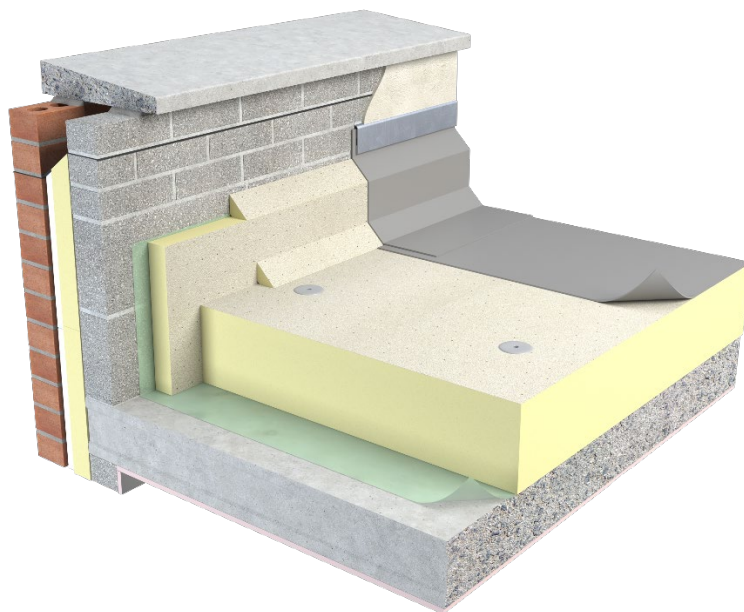
Figure 1: Unilin Insulation FR/MG onto Concrete Deck
