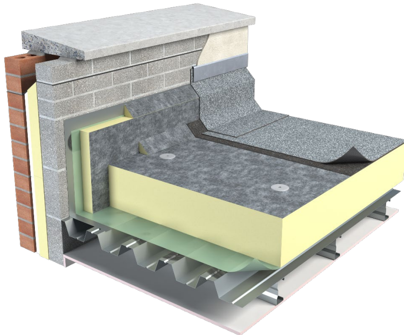
Figure 1: Unilin Insulation FR/BGM onto Metal Deck
