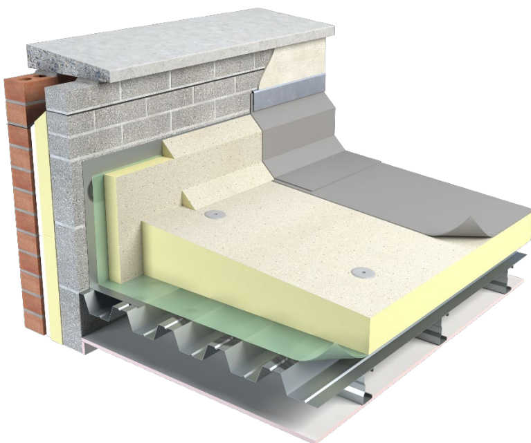
Figure 1: Unilin Insulation TR/MG onto Metal Deck
