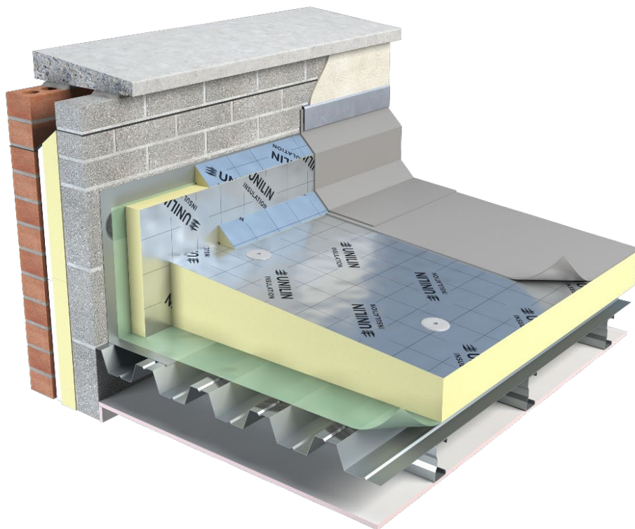
Figure 3: Unilin Insulation TR/ALU onto Metal Deck
