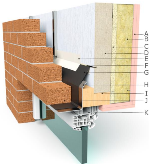
A Plasterboard G DPC B Rockwool H Steel Lintel C Closed Cell Insulation I Timber Batten D P.I.R./Phenolic Insulation J External Masonry Wall E Tape K Window F PU Foam
