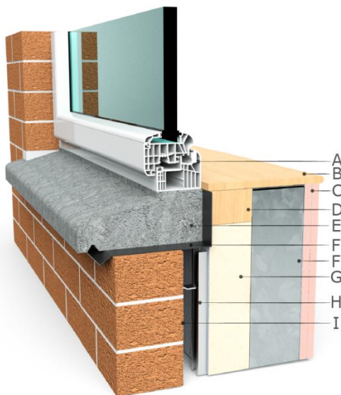
A Window F Steel Stud B Timber Cillboard G P.I.R./Phenolic Insulation C Plasterboard H Stainless Steel Wall Channel D Timber Batten I External Masonry Wall E Cement Cill
