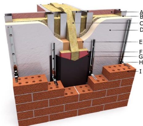
Figure 13: Party wall detail (Option 1) at junction with external masonry wall
