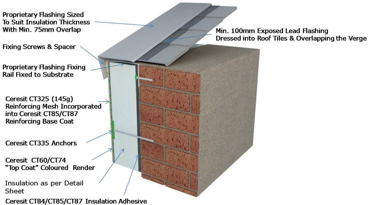
Figure 9: Verge Trim Detail
