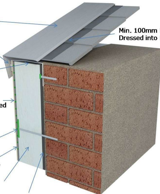
Figure 9: Verge Trim Detail
