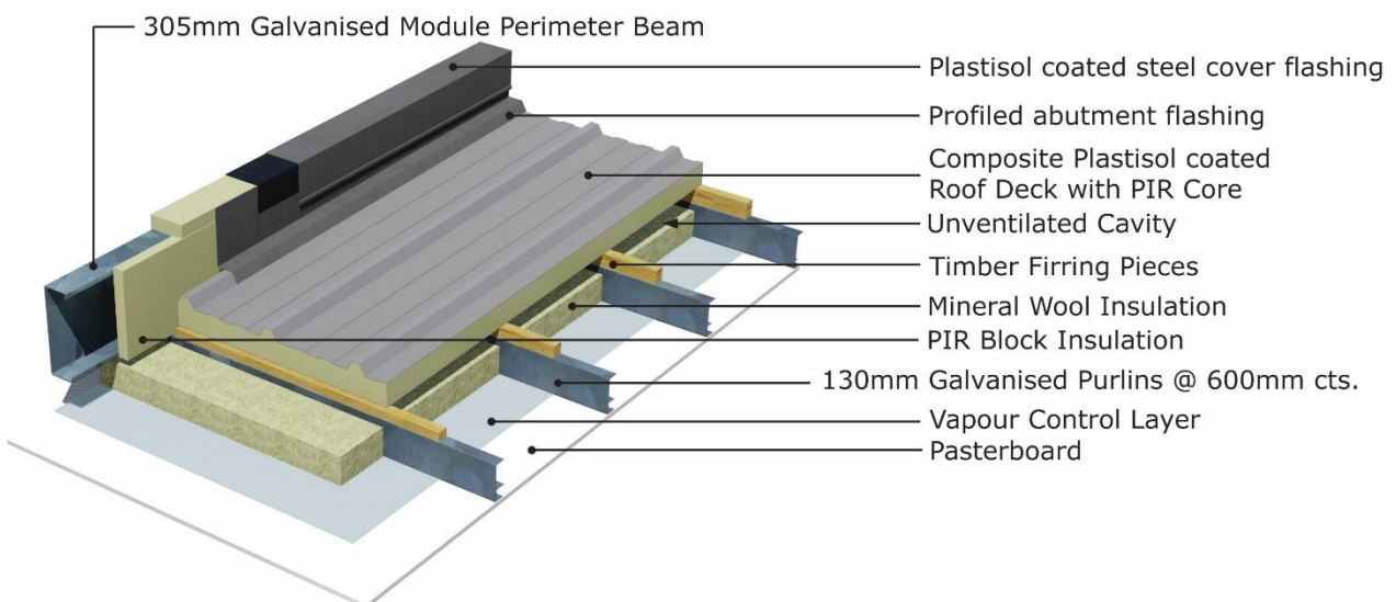
Figure 4 - Roof Type 2
