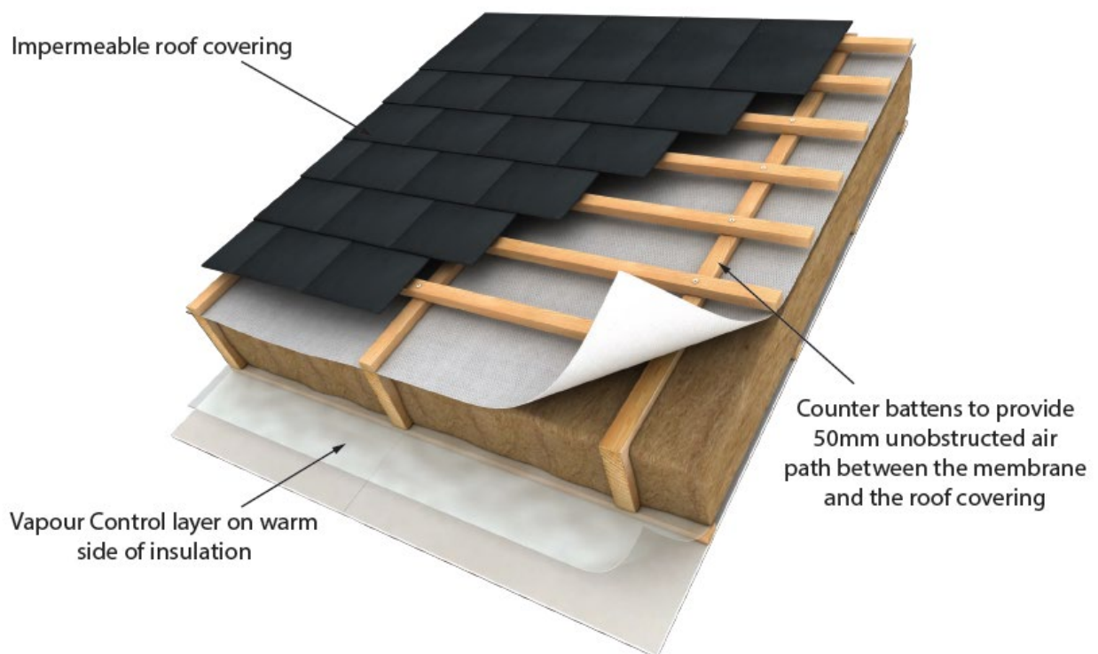
Figure 2: Warm Roof detail with impermeable roof covering
