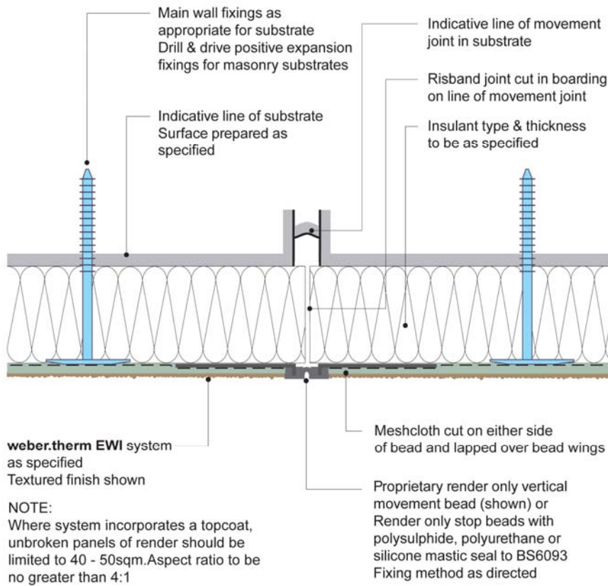
Figure 7: Movement Joint
